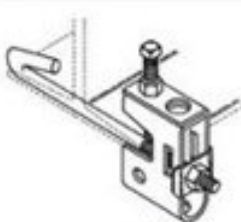
Figure 6: Example of beam clamp retaining strap (1) (Source: ACME Construction Supply Co.)
